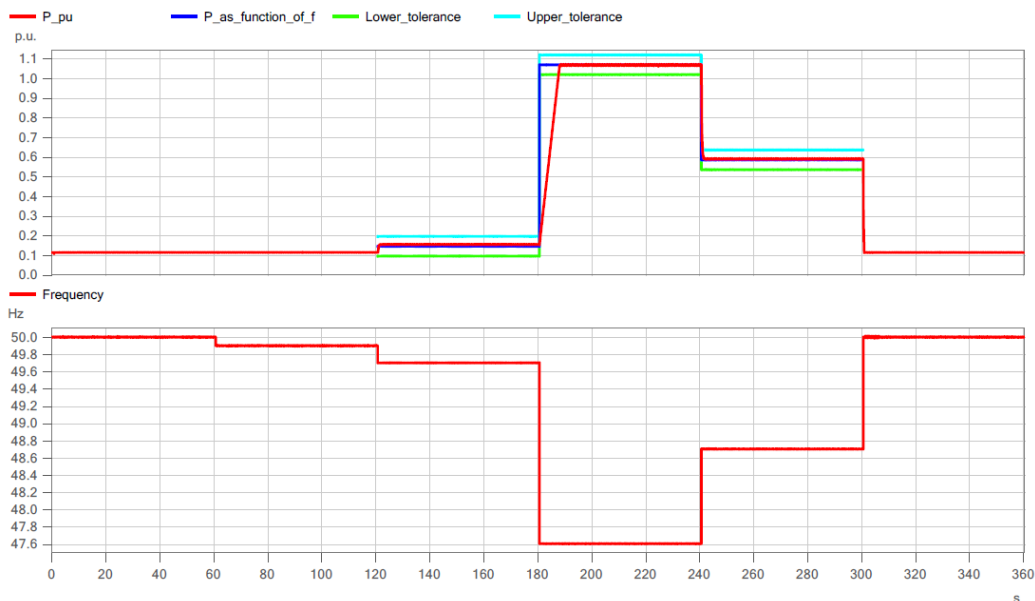
Figure 5-8 LFSM-U test results, showing input frequency steps (lower plot) and the response in active power output (upper plot), droop: 5%, activation threshold: 49.8 Hz /1/
