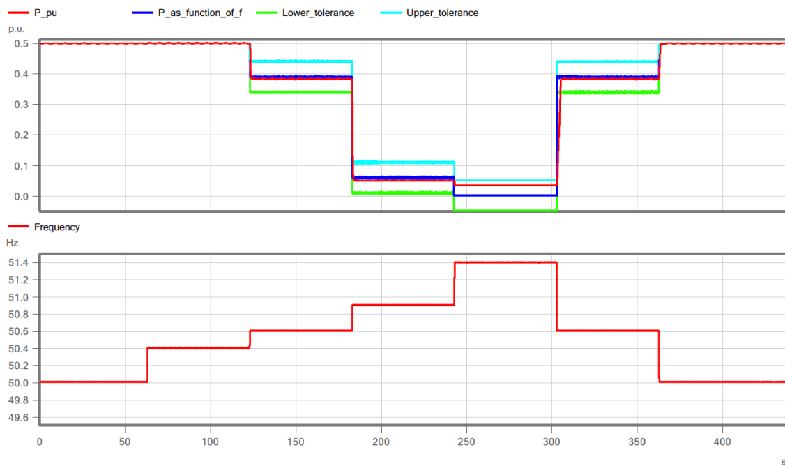
Figure 5-6 LFSM-O test results, showing input frequency steps (lower plot) and the response in active power output (upper plot), droop:2%, activation threshold: 50.5 Hz /1/
