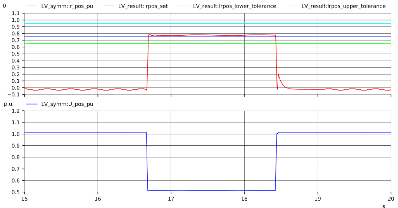
Figure 5-12 Test no. 33 (3-phase, full-load, fault voltage 50 p.u. of Un, k=2), showing positive sequence response /1/.
