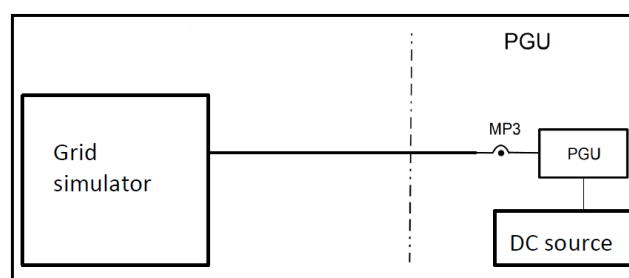
Figure 4-1 Single line diagram of the test setup
